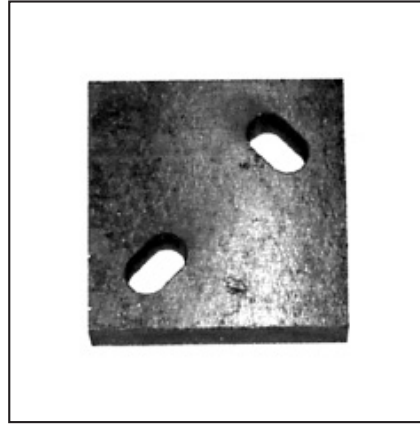
2_ Mounting plate for Square post 45mm x 45mm [1 3/4" x 1 3/4"]
